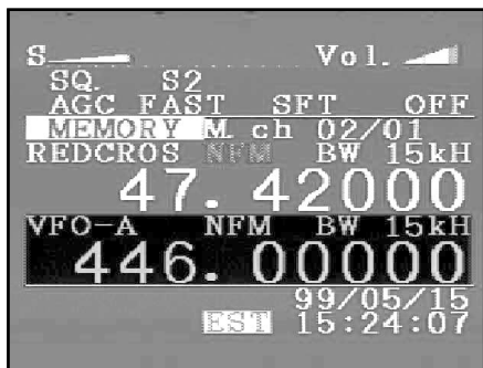
Figure 6—The display screen of the AR7000B showing the contents of memory channel 2 of bank 1. Graphic representations of the signal strength and volume level appear at the top of the screen. The selected squelch level is indicated in S units.
